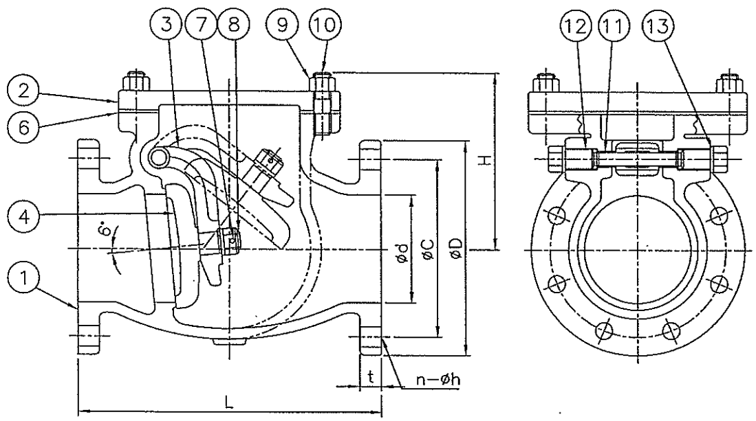
Dimension [Unit: mm]
